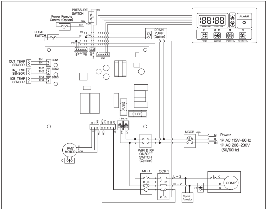
Figure 13 - Circuit Wiring Diagram (WPC-3000,5000)
