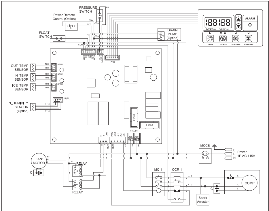
Figure 14 - Circuit Wiring Diagram (WPC-4000)
