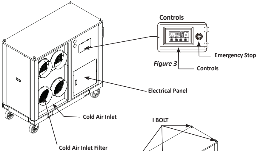
Figure 2 Front and Right Side View
